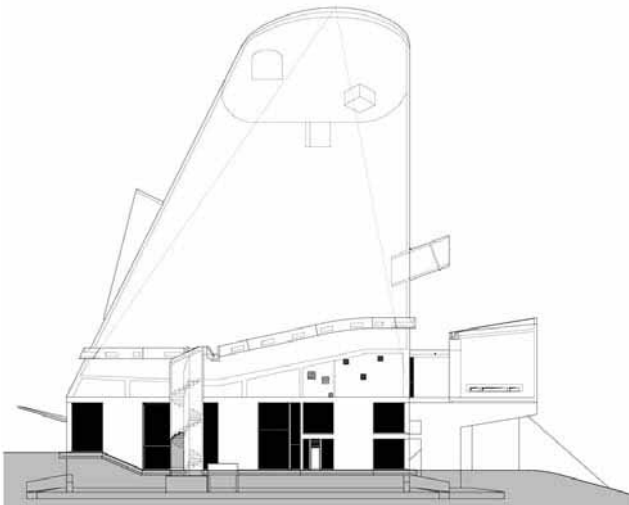
NORTH FACADE
