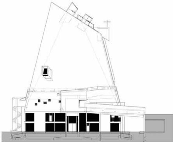
WEST FACADE
