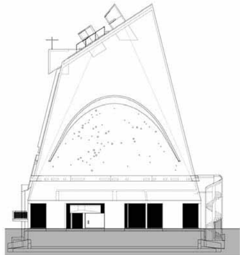
EAST FACADE
