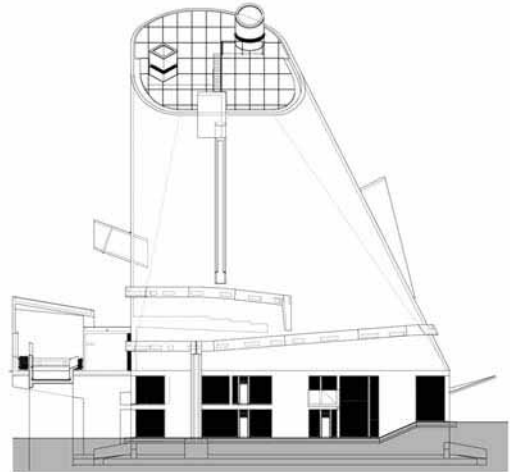
SOUTH FACADE
